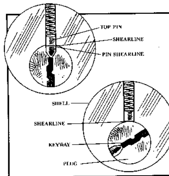
Figure 2. The pin tumbler lock, front view.
