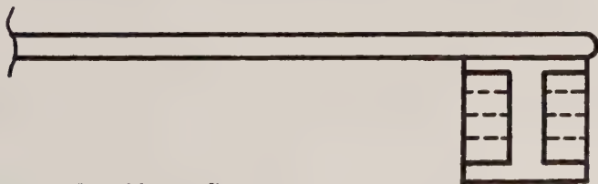
Figure 6: Possible warding cuts.
