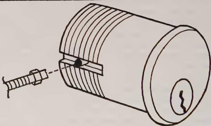
Figure 58: Tip of cylinder set screw sheared off by turning.
