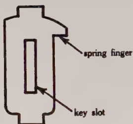
Figure 13: An individual disc tumbler.
