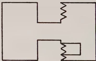
Figure 51: Serrated cut lever tumbler and stump.
