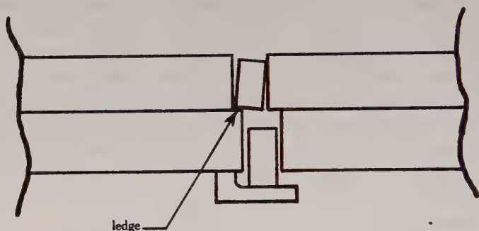
Figure 39: Top pin trapped by plate misalignment.
