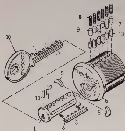
Figure 54: Medeco sidebar lock diagram
